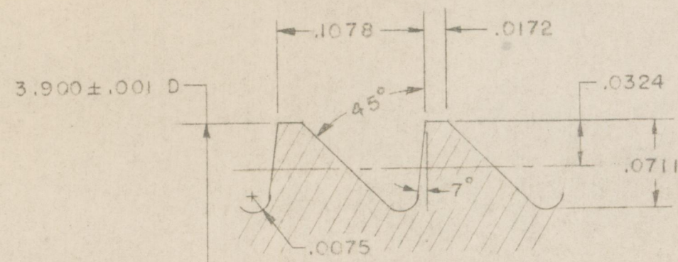
BUTTRESS THREAD DETAIL
